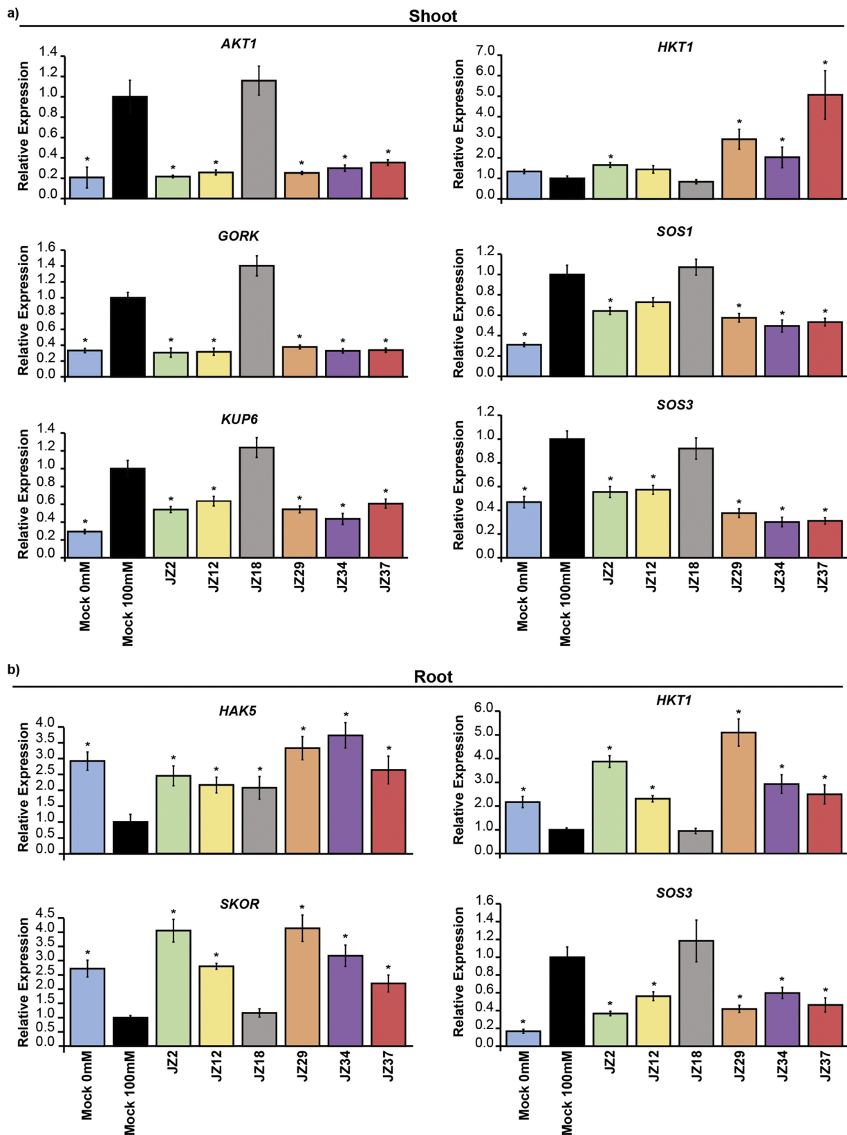
Fig. 5. Effects of bacterial inoculation on the expression of genes involved in sodium and potassium transport in A. thaliana shoot and roots under salinity stress. Normalized qPCR expression levels of genes involved in potassium (left) and sodium (right) transport in the shoots (a) and roots (b); AKT1 ( K^+ Transporter 1), GORK (Gated Outwardly-Rectifying K^+ Channel), KUP6 ( K^+ Uptake Permease 6), HKT1 (High-Affinity K^+ Transporter 1), SOS1 (Salt Overly Sensitive 1), SOS3 (Salt Overly Sensitive 3), HAK5 (High Affinity K^+ Transporter 5) and SKOR (Stellar K^+ Outward Rectifier). RNA was extracted from the shoots or roots of A. thaliana 16 DAI with or without bacteria on \frac{1}{2} MS + 100 mM NaCl and 0 mM NaCl as non-stress control. Data are means of 3 biological replicates collected from 4 to 6 different plants per replicate and are normalized to non-inoculated control plants (100 mM NaCl). Error bars represent standard error of the mean (SEM). Asterisks indicate significant differences between mock (100 mM NaCl) and bacteria-inoculated (100 mM NaCl) or non-stressed mock (0 mM NaCl) plants (regulation threshold \geq 1.5 , p \leq 0.05 ).
