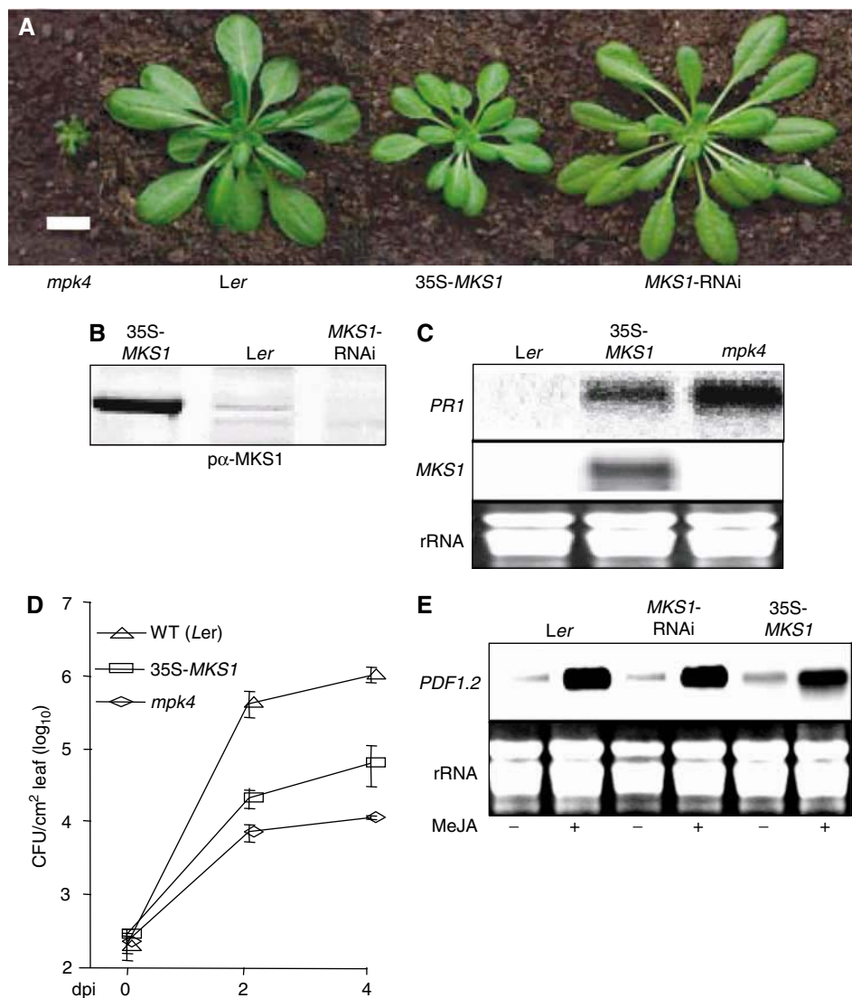
Figure 4 Effects of MKS1 over- and underexpression. (A) Phenotypes of mpk4 , wild type ( Ler ) and transgenic ( Col ) overexpressing MKS1 (35S-MKS1) or underexpressing MKS1 (MKS1-RNAi). The size bar is 2 cm. (B) Immunodetection with \alpha -Pep22 antibody of MKS1 in extracts from 35S-MKS1, wild type ( Ler ) and MKS1-RNAi. (C) RNA blot detection of PR1 mRNA in 35S-MKS1, mpk4 and wild-type Ler . (D) Growth of P. syringae pv. tomato DC3000 in mpk4 , 35S-MKS1 and Ler . (E) Detection of PDF1.2 mRNA in wild type ( Col ), MKS1-RNAi and 35S-MKS1 following MeJA (+) and mock (-) treatments.
