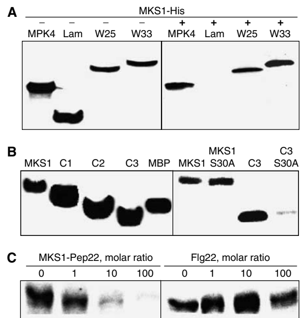
Figure 1 MKS1 interactions and phosphorylation in vitro . (A) MKS1 interactions with MPK4, W25 and W33 using N-terminal 6xHis-tagged MKS1 (His-MKS1) purified from E. coli . ^{35} S-methionine-labeled MPK4, W25 or W33 was incubated without (–) or with (+) nickel-agarose-coupled His-MKS1. Human lamin (Clontech) was a negative control. (B) Left: Phosphorylation of full-length recombinant MKS1, C-terminal MKS1 truncations (C1–C3) and myelin basic protein (MBP) as positive control. HA-tagged MPK4 (HA-MPK4) was immunoprecipitated (IP) from complemented mpk4 transgenic plants. Right: In vitro kinase assays with mutated full-length MKS1 (MKS1 S30A) and mutated C3 (C3 S30A). (C) Phosphorylation of full-length MKS1 and increasing molar ratios of a 22-amino-acid, MKS1-derived peptide, Pep22 (left; Supplementary Figure S1) and the 22-amino-acid flagellin elicitor Flg22 (right).
