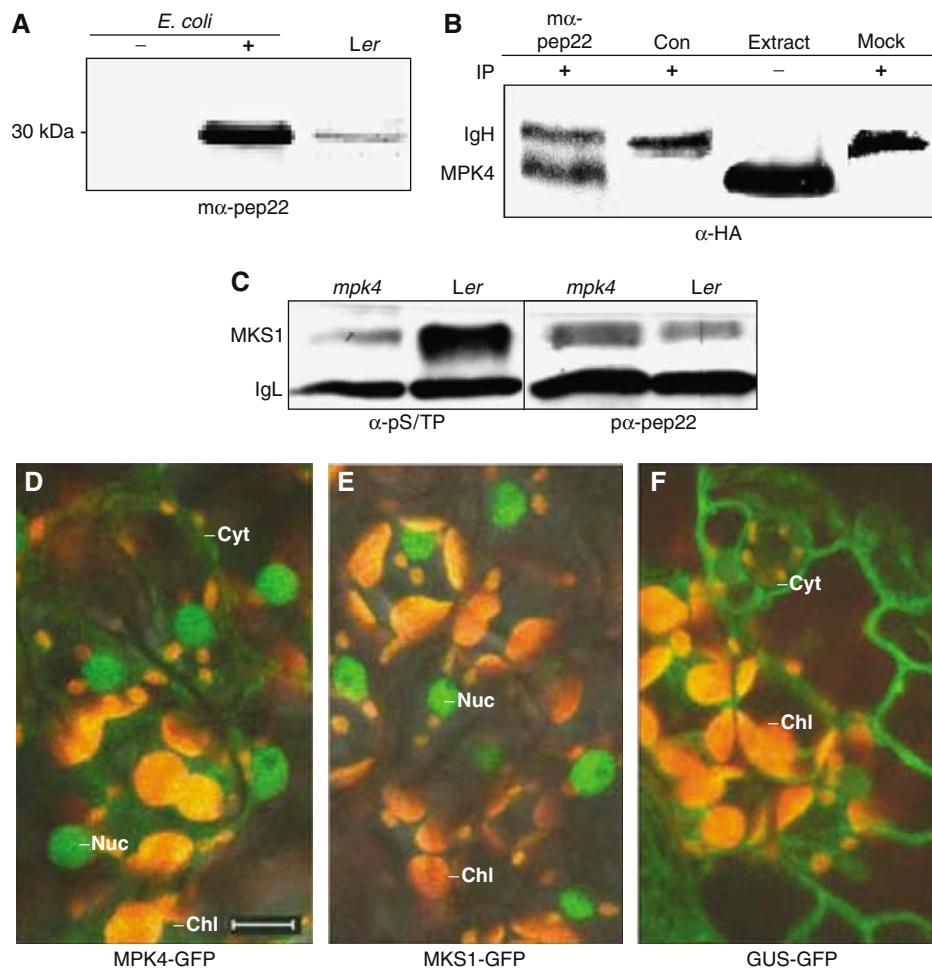
Figure 3 MKS1 interaction, phosphorylation and localization in vivo . (A) Immunodetection of MKS1 in E. coli extracts before (–) and after (+) IPTG induction, and from extracts of leaves ( Ler ) by a monoclonal anti-Pep22 antibody ( m\alpha -pep22) recognizing a protein of the predicted size of MKS1 (~28 kDa). (B) Immunodetection of HA-MPK4 by anti-HA antibody ( \alpha -HA) in immunoprecipitates from plant extracts with m\alpha -pep22 (lane 1), negative control monoclonal antibody (Con; lane 2) or in mock immunoprecipitation lacking extract (lane 4). MPK4 from plant extracts is shown (raw extract; lane 3). MPK4 and immunoglobulin heavy chain (IgH) are indicated. (C) Immunodetection of MKS1 following immunoprecipitation with m\alpha -Pep22 from Ler or mpk4 extracts. MKS1 is detected with an anti-phosphoserine/phosphothreonine antibody ( \alpha -pS/TP) and polyclonal anti-Pep22 antibody ( p\alpha -pep22). MKS1 and immunoglobulin light chain (IgL) are indicated. In planta localization in mesophyll cells of (D) MPK4-GFP, (E) MKS1-GFP and (F) GUS-GFP fusion proteins. Cyt: cytoplasm; Nuc: nuclei; Chl: chloroplast (orange autofluorescent); – 10 \mu m size bar.
