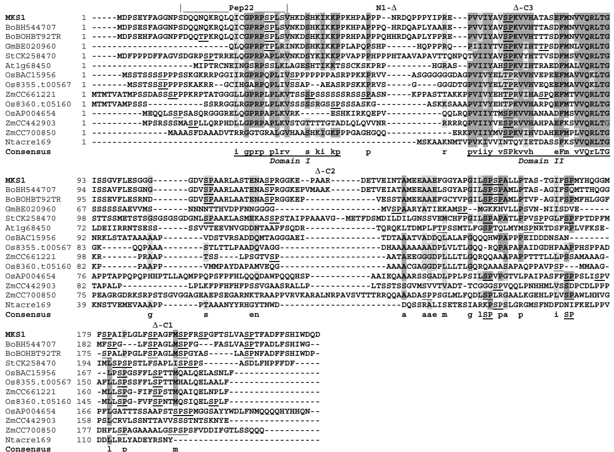
Figure 2 MKS1 and homologs. DNA and amino-acid sequences of MKS1 (At3g18690) were used to query databases at www.ncbi.nlm.nih.gov/BLAST for proteins similar to MKS1. Protein sequences of selected accessions were aligned at clustalw.genome.jp and identical/similar residues highlighted at www.ch.embnet.org/software/BOX_form.html . Putative MAP kinase phosphorylation sites (S/TP) are underlined. The sequence of the Pep22 peptide is indicated by an overbar. The ends of an N-terminally truncated (N1) and three C-terminally truncated (C1-3) MKS1 versions described in the text are noted above the MKS1 sequence. Putative domains I and II are underlined in the consensus. Species abbreviations are as follows: At: Arabidopsis thaliana ; Bo: Brassica oleracea ; Gm: Glycine max ; St: Solanum tuberosum ; Os: Oryza sativa ; Nt: Nicotiana tabacum ; Zm: Zea mays . Similar plant proteins not aligned here include BM340911, CAD40925, CC613160, CC635639, AI390921, AL138658, T46022, AP004654, AP003260, AC143340 and Arabidopsis At1g21326, At2g41180, At2g44340, At2g42140 and At3g56710 (Sig1; Morikawa et al, 2002).
