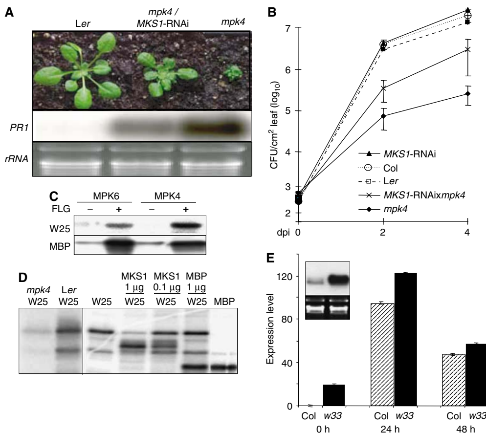
Figure 5 Suppression of mpk4 by MKS1 -RNAi, WRKY phosphorylation and w33 phenotype. (A) Top: Phenotypes of wild type ( Ler ), mpk4 carrying MKS1 -RNAi ( mpk4/MKS1 -RNAi) and mpk4 . Bottom: Detection of PR1 mRNA in wild type ( Ler ), mpk4/MKS1 -RNAi and mpk4 versus rRNA loading control. (B) Growth of P. syringae pv. tomato DC3000 in wild types Ler and Col , mpk4 , MKS1 -RNAi and mpk4/MKS1 -RNAi. (C) Phosphorylation of full-length W25 by immunoprecipitation of MPK6 or MPK4 from Arabidopsis cells without (-) or with (+) treatment with flagellin. (D) Phosphorylation of N-terminal region of W25 with MPK4 immunoprecipitation from mpk4 or Ler (left) and of W25, MKS1 and MBP with immunoprecipitation of MPK4 -HA (right). (E) RNA blot (inset) and real-time PCR detection of PR1 mRNA in Col and w33 before (0 h and inset) or after infiltration with DC3000.
