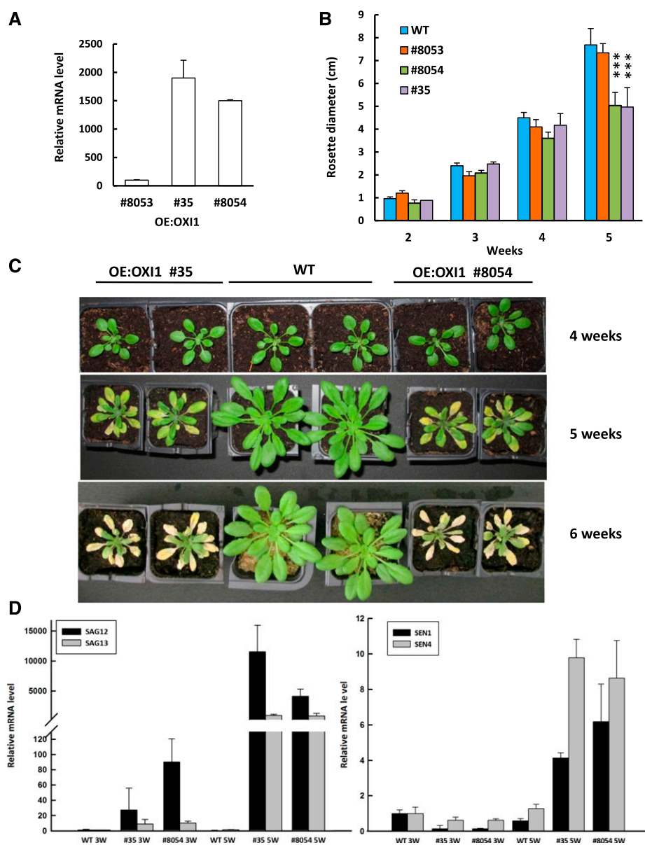
Figure 1. Overexpressing OX11 in Arabidopsis leads to an accelerated senescence phenotype. A , RT-qPCR analysis of the expression levels of OX11 in three OE: OX11 lines (35, 8053, and 8054) relative to the wild type. n = 3 biological replicates. B , Growth curves of wild-type plants and the three OE: OX11 lines ( n = 3 ). Plants were grown under short-day conditions (photoperiod, 8 h). *** P < 0.001 compared to the wild type, as determined by Student's t test. C , Phenotype of wild-type and OE: OX11 plants at different ages (4, 5, and 6 weeks). D , Senescence marker genes SAG12 , SAG13 , SEN1 , and SEN4 in leaves of wild type and OE: OX11 lines 35 and 8054 aged 3 weeks and 5 weeks (3W and 5W, respectively). RT-qPCR measured expression levels are normalized to the wild-type levels at week 3 ( n = 3 ).
